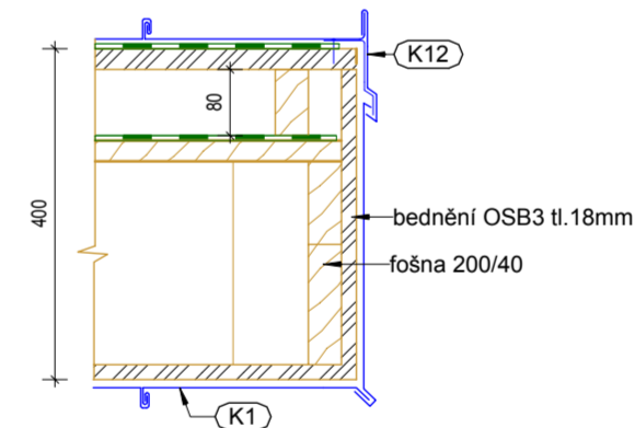
Detail 6 ( 1:10 )
