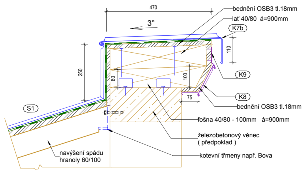
Detail 4a ( 1:10 )
