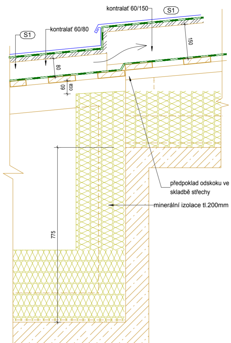
Detail 2 ( 1:10 )
