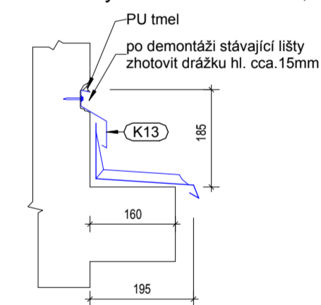
Detail 7 ( 1:10 )
