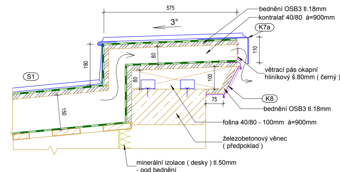
Detail 3 ( 1:10 )
