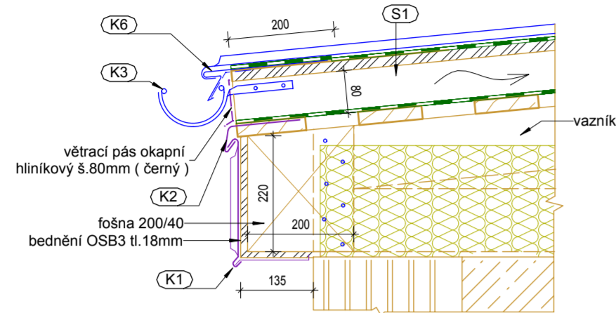
Detail 1 ( 1:10 )
