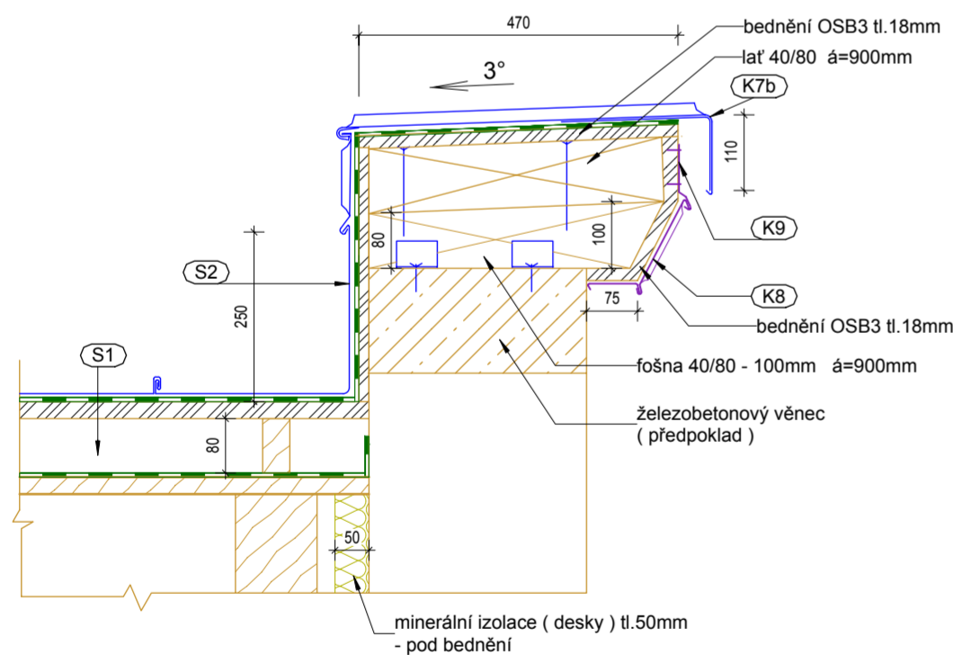
Detail 4 ( 1:10 )
