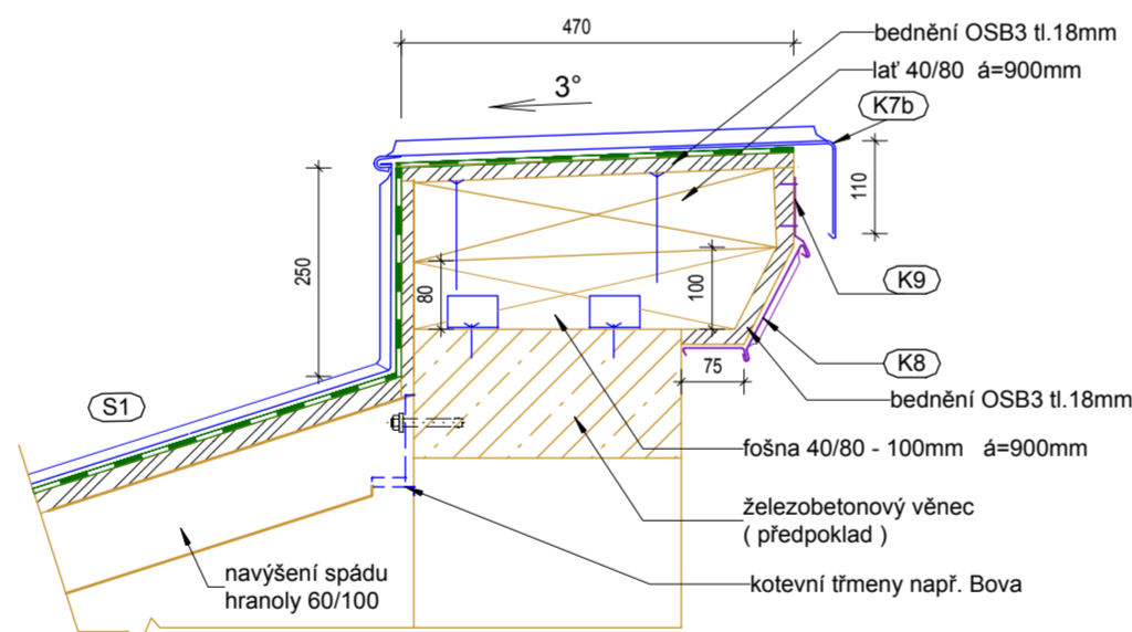
Detail 4a ( 1:10 )
