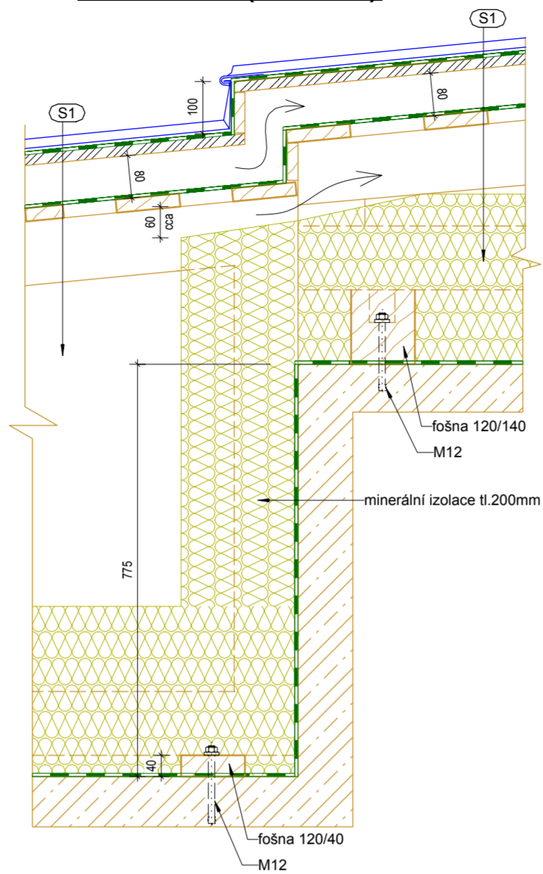
Detail 2 ( 1:10 )
