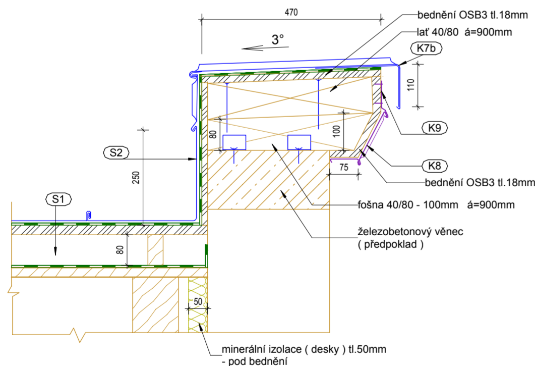
Detail 4 ( 1:10 )
