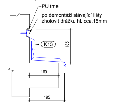
Detail 7 ( 1:10 )
