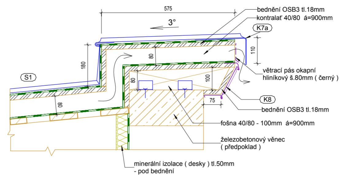
Detail 3 ( 1:10 )
