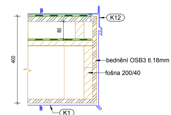
Detail 6 ( 1:10 )
